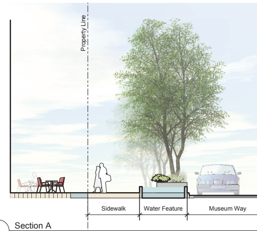
1 Section A 1:100
